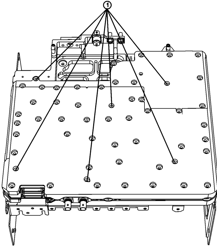
Figure 22 Replace Screws and SMB Cable
