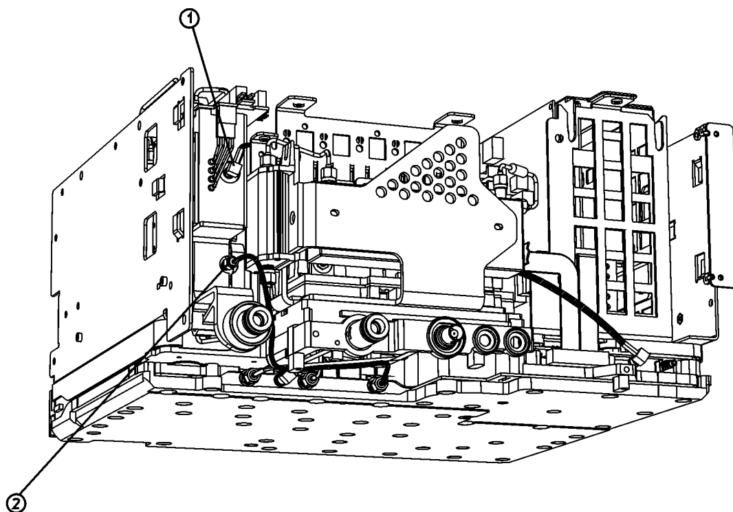
Figure 23 Replace Tracking Generator Cables
