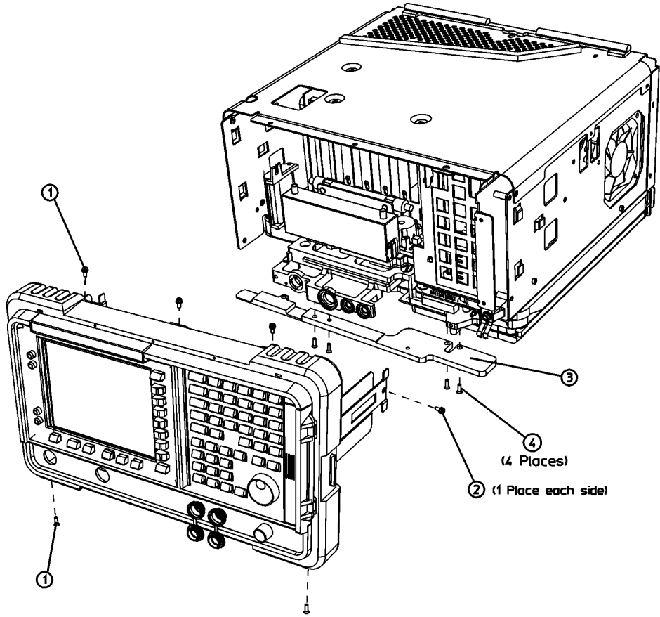
Figure 25 Front Frame Assembly Replacement
